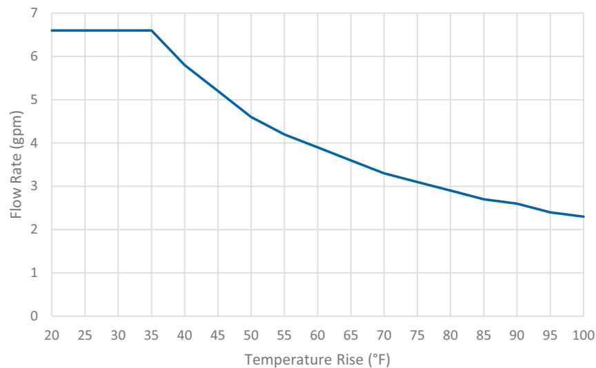
110U Output Temp vs. GPM
